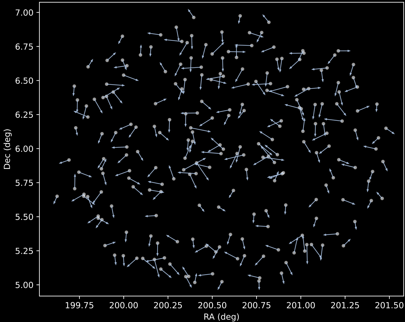
GALAH DR4 Cluster 1 Proper Motion Vectors (n=221)
