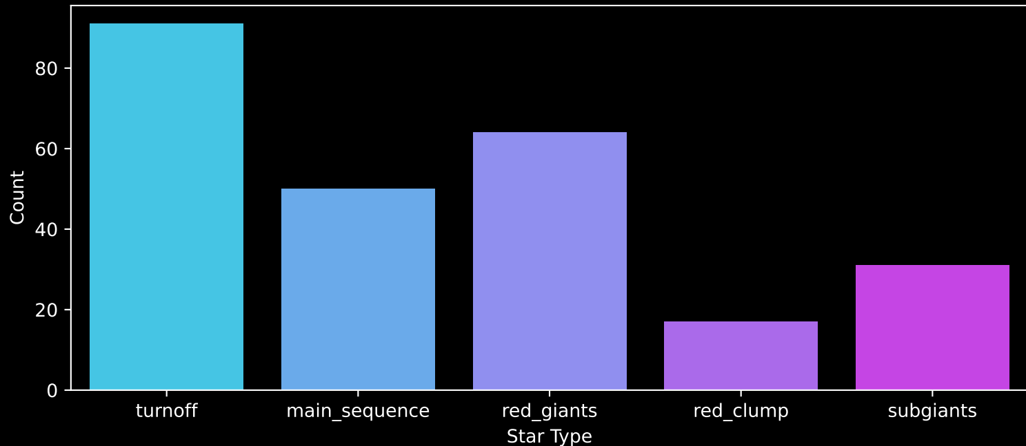
GALAH DR4 Field: [9400] Count plot of Star Type
