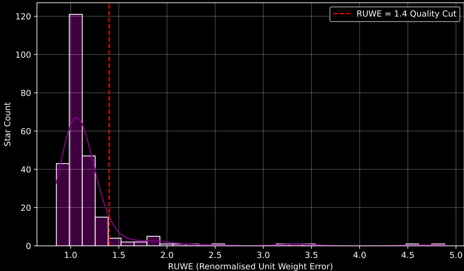
GALAH DR4 Field [9400] RUWE Distribution (n= 248)
